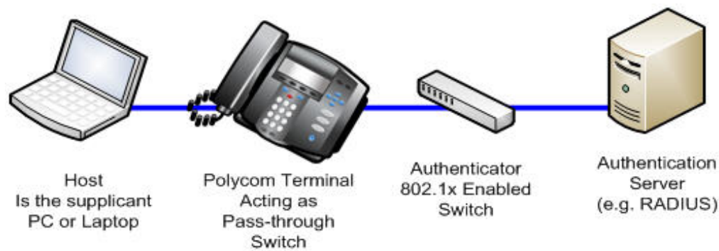
Figure 9-1: A Polycom Terminal Acting as a Pass-Through Switch
